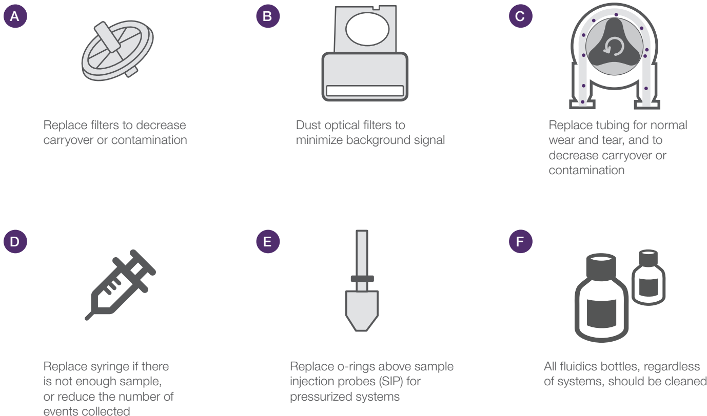
Figure 23. Fluidics maintenance. (A–F) Clean or replace flow cytometry instrument parts to maintain normal instrument performance and minimize carryover, background noise, and microbial contamination.
