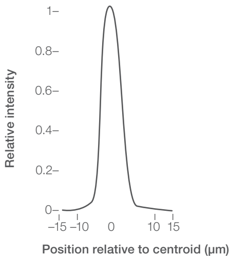
Figure 12. Laser profiles. (A) In a Gaussian emission profile, photons are dense and most intense in the center. (B) A flat-top beam intensity profile covers a larger and flatter area. Cells pass through a wider apex to emit fluorescence.
