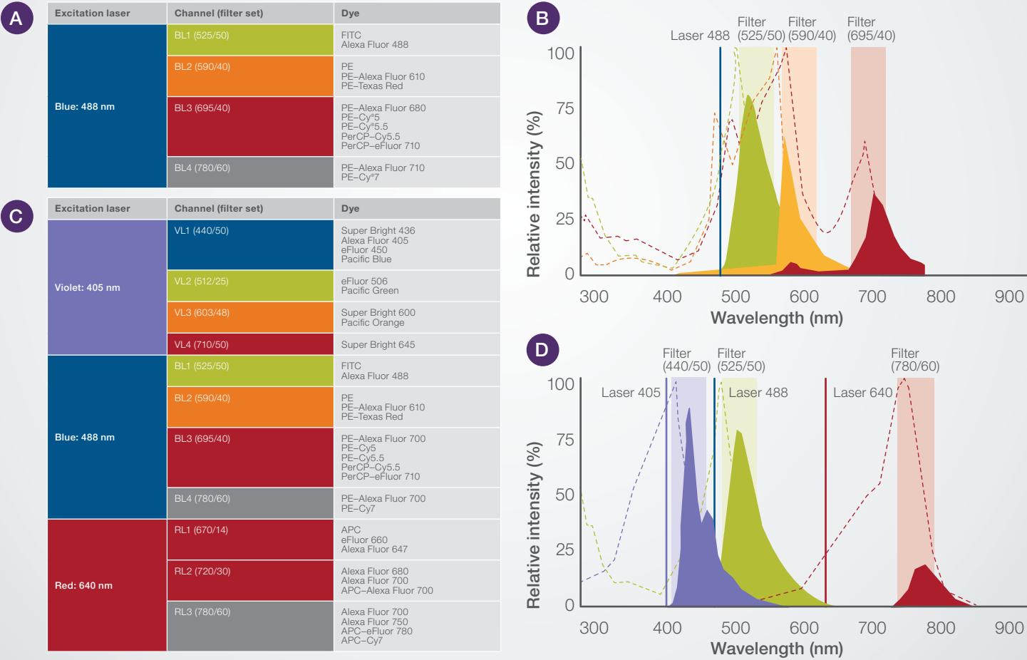
Figure 20. Channels. (A) A one-laser system can have multiple channels. (B) The emitted light overlaps and requires compensation. (C) A 3-laser system will have more channels because there are more detectors. (D) The channels are spread out, allowing for more fluorophore options and less compensation.
