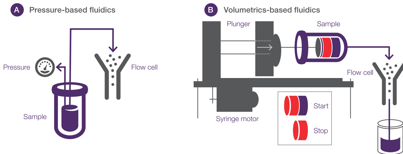
Figure 2. Systems for sample entry into the flow cytometer. (A) Pressure-based fluidics rely on the pressure difference between the sample fluid stream and the sheath fluid surrounding the sample stream. (B) Volumetrics-based fluidics provide the ability to obtain concentration and count measurements, since the exact sample volume can be measured.
