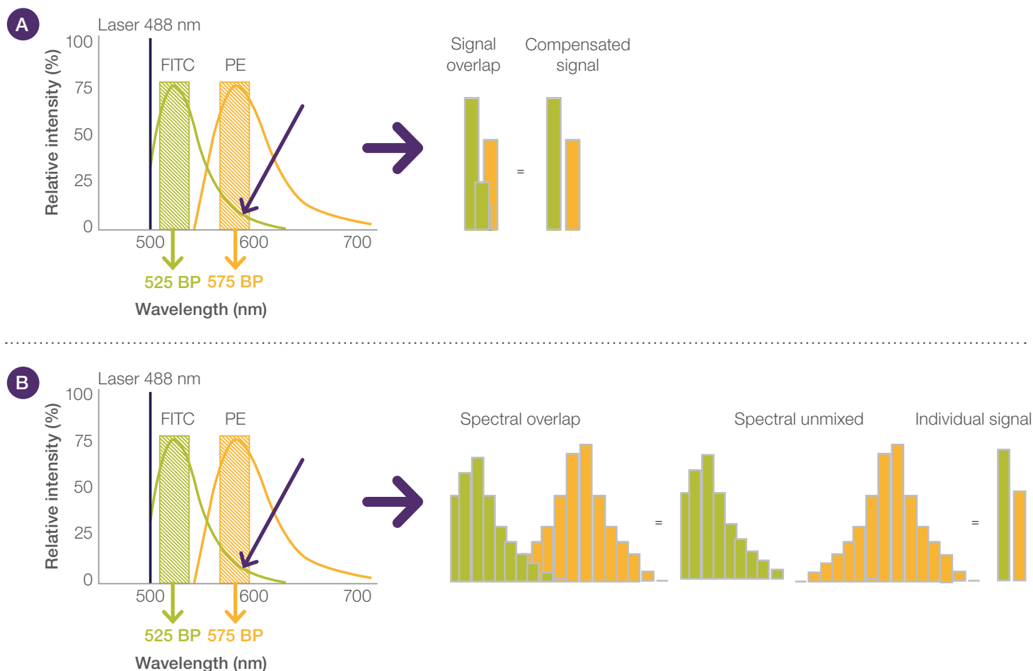
Figure 19. Compensation techniques. (A) Traditional compensation uses well-researched sets of algorithms to analyze data from fluorophores, negative gating, or unstained controls to process overlapping emission into a single color. (B) Spectral unmixing uses sets of algorithms such as constrained Poisson regression or nonnegative matrix factorization to process light into a single color.
