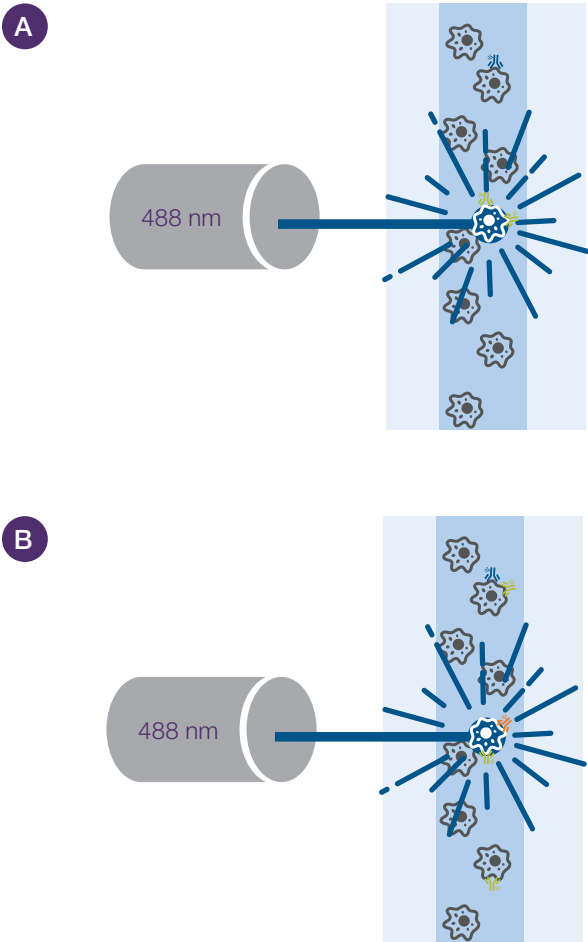
Figure 14. Fluorescence emission. (A) Excited fluorophores emit light in a limited range of wavelengths. (B) Some fluorophores can have overlapping emission spectra.
