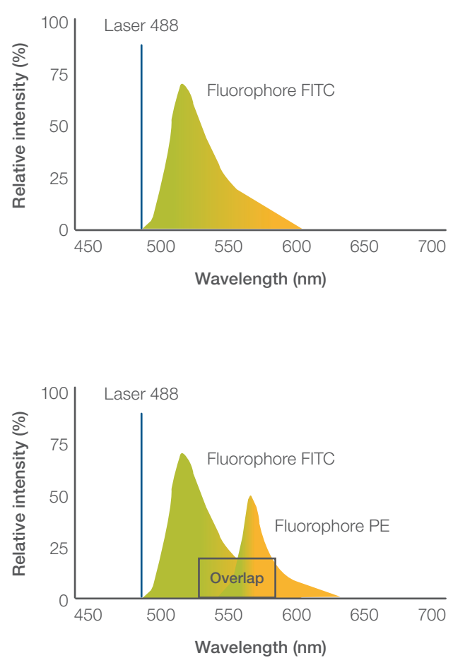
Figure 14. Fluorescence emission. (A) Excited fluorophores emit light in a limited range of wavelengths. (B) Some fluorophores can have overlapping emission spectra.
