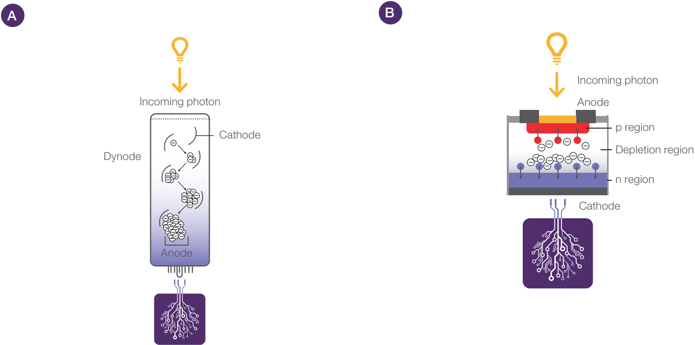
Figure 16. Components for emission detection. (A) PMTs capture and multiply the signal emitted by a fluorophore. (B) APDs capture photons on a semiconductor and then multiply the signal.
